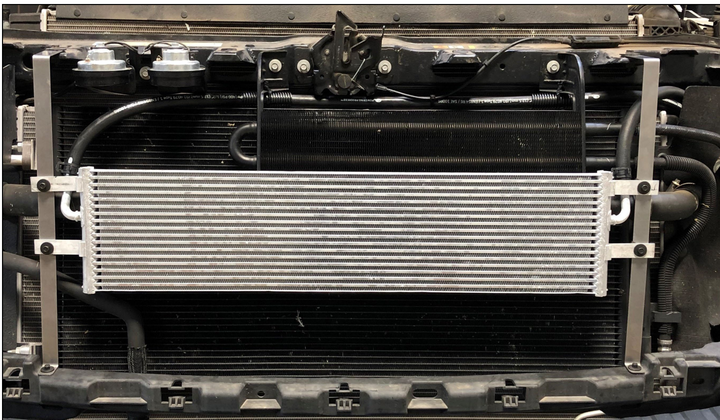
FIGURE 14 – Cooler and Hoses Installed, Routed and Secured
